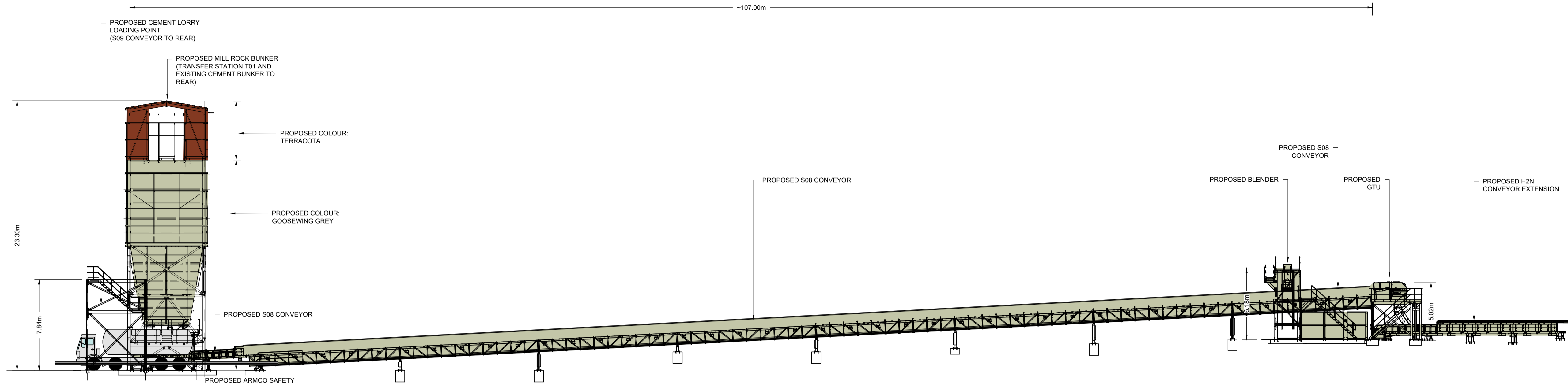
ELEVATION A-A - OVERVIEW OF ENTIRE PROPOSED INFRASTRUCTURE
