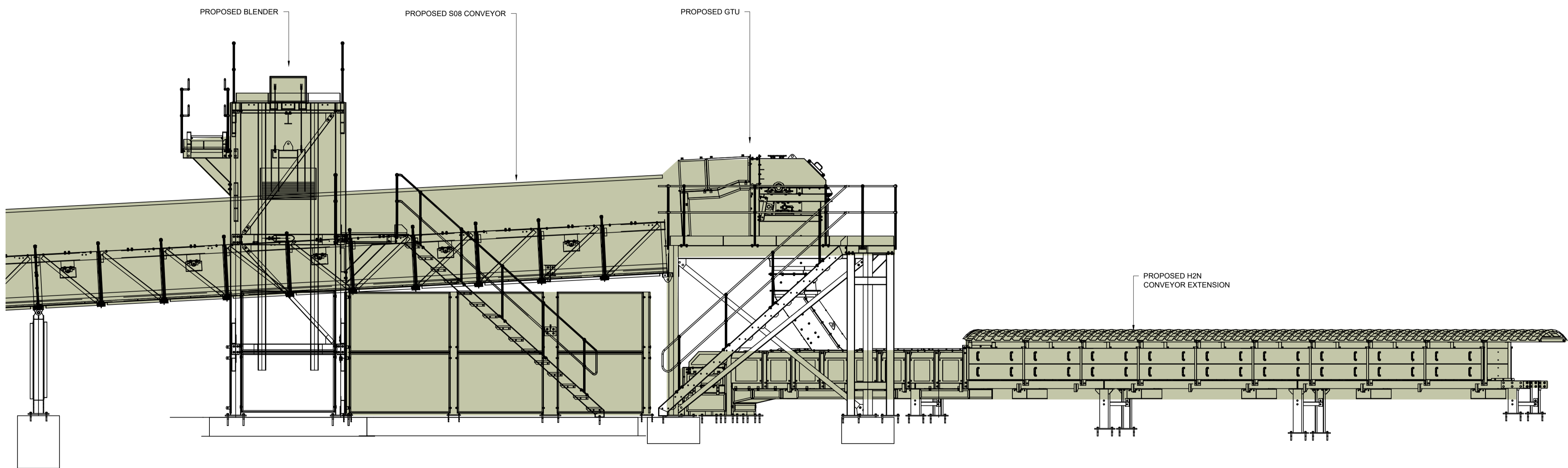
ELEVATION C-C - ON PROPOSED BLENDER AND H2N CONVEYOR EXTENSION
